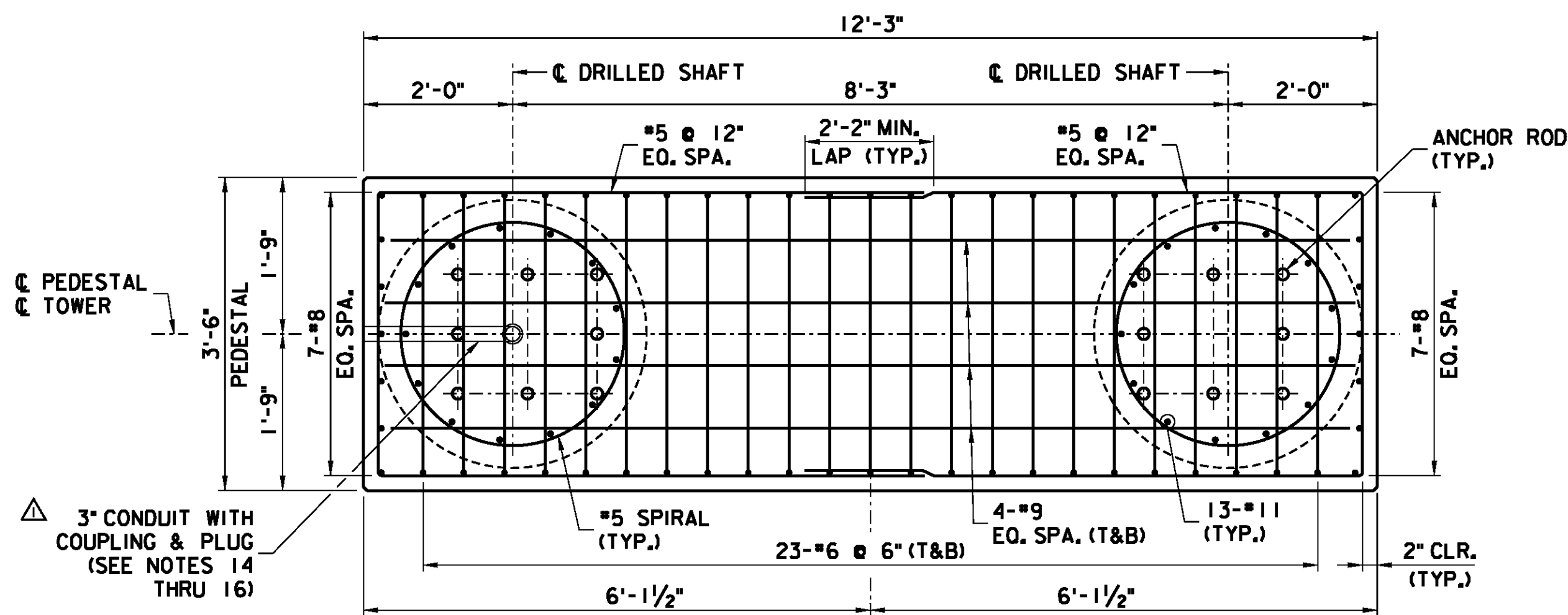
PLAN VIEW A-A
