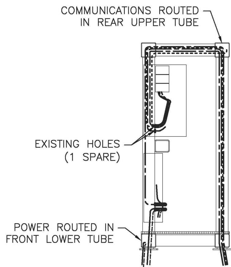
SIDE VIEW
