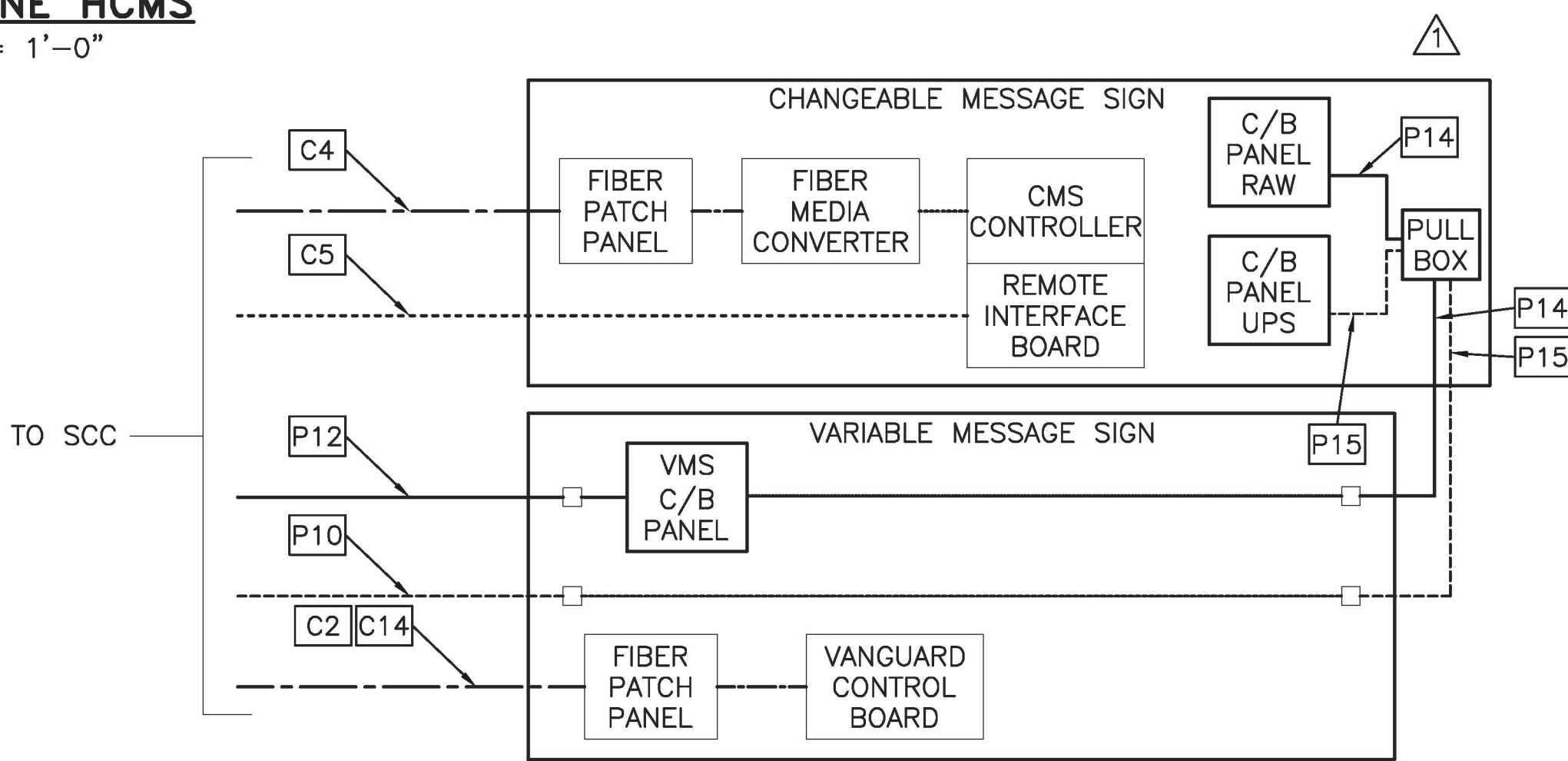
SINGLE MAINLINE HCMS WIRING DIAGRAM
