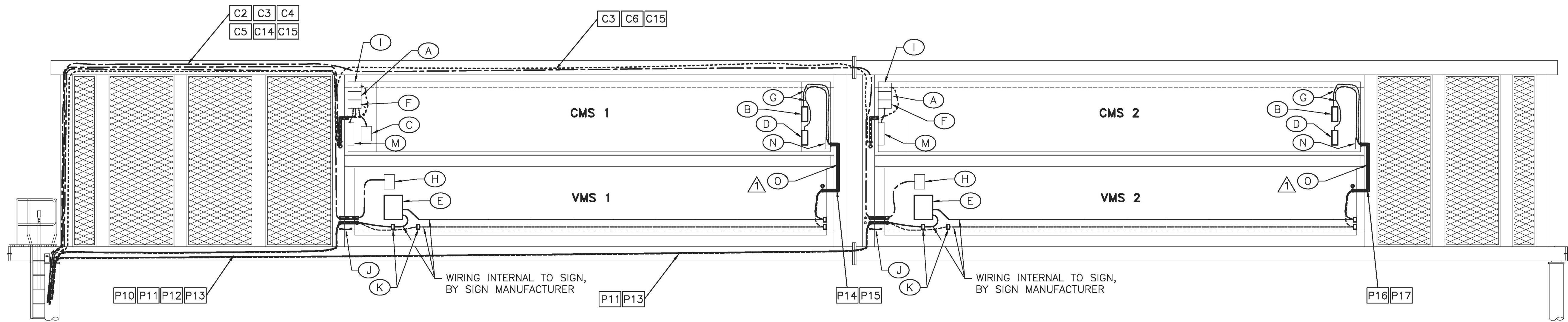
REAR ELEVATION
