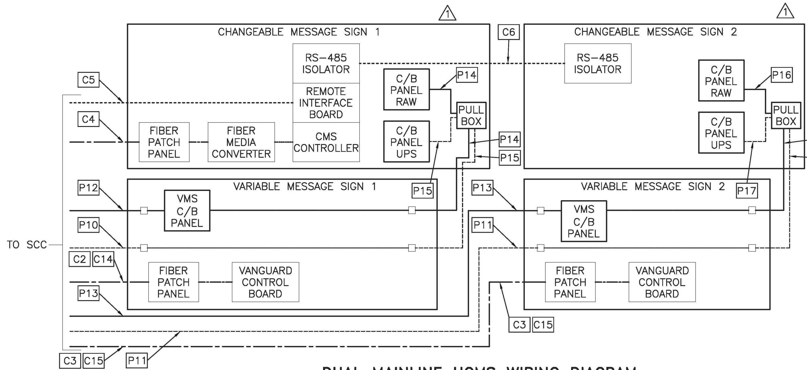
DUAL MAINLINE HCMS WIRING DIAGRAM
