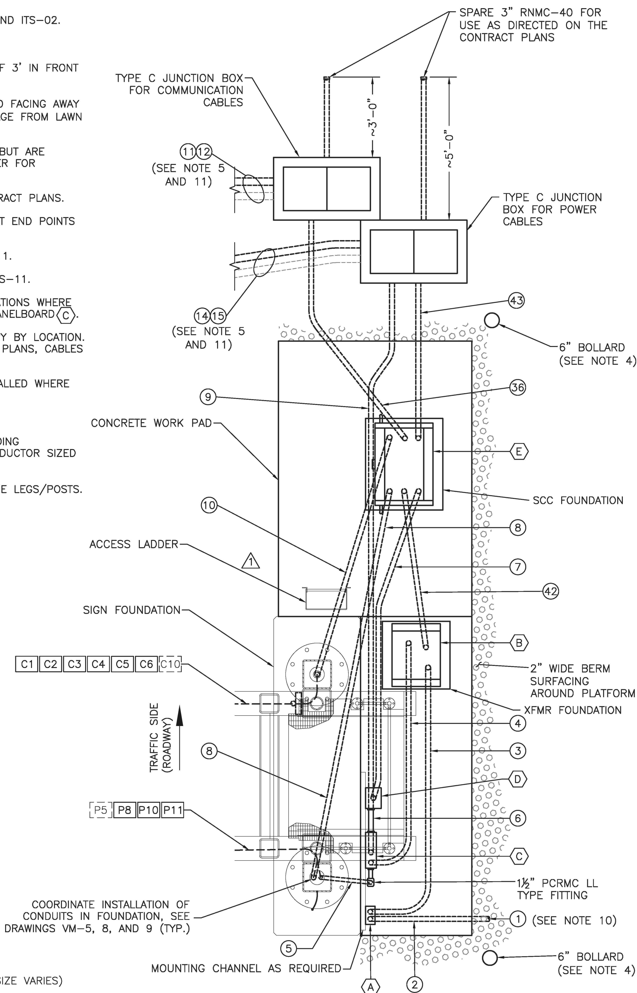
OUTER ROADWAY – SCC INSTALLATION PLAN SCALE: \frac{1}{2}" = 1'-0"
