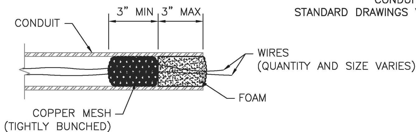
CONDUIT END RODENT BLOCKING DETAIL NOT TO SCALE
