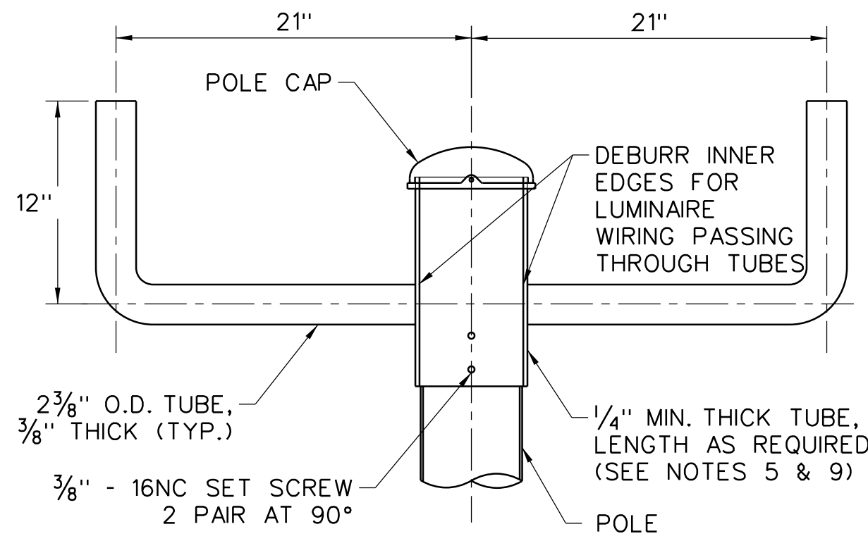
LUMINAIRE MOUNTING ASSEMBLY TYPE V2
