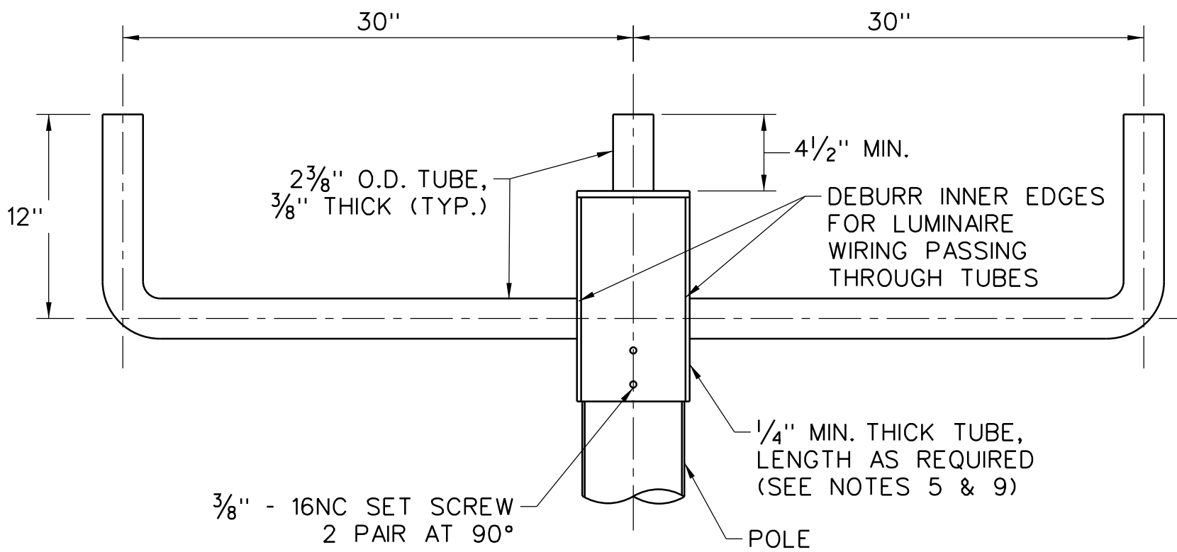
LUMINAIRE MOUNTING ASSEMBLY TYPE V3
