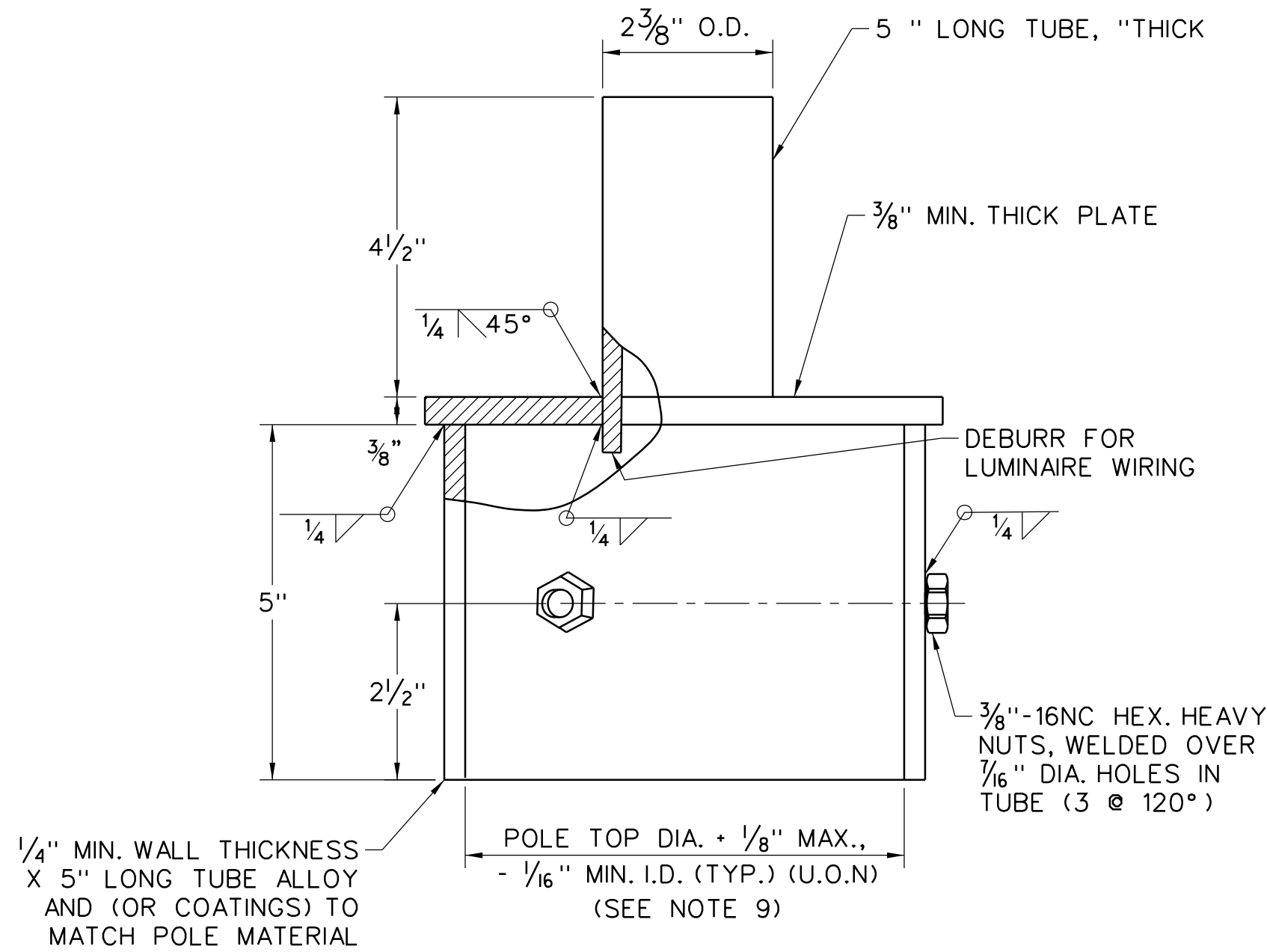
LUMINAIRE MOUNTING ASSEMBLY TYPE V
