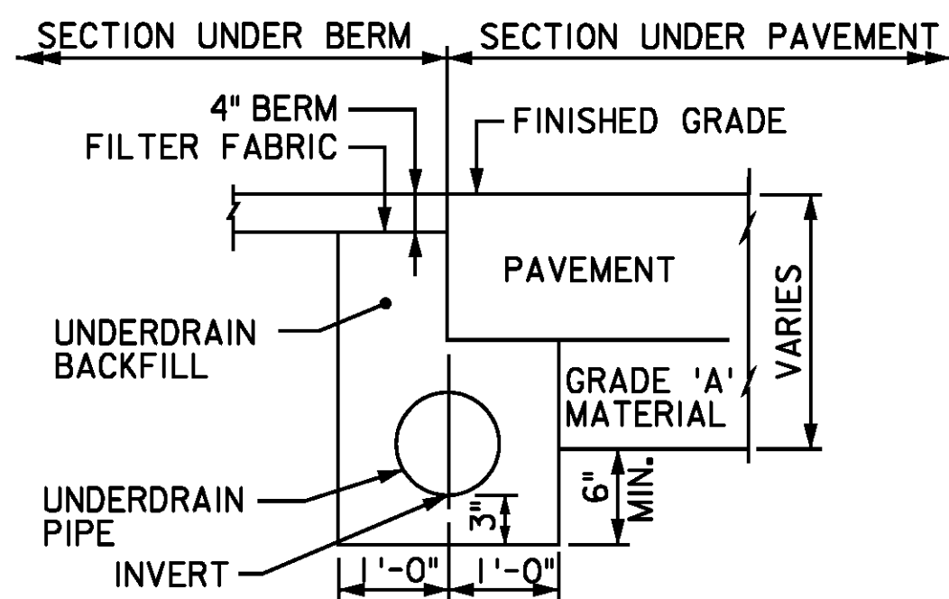
PIPE UNDERDRAIN (8" PIPE UNLESS OTHERWISE NOTED)
