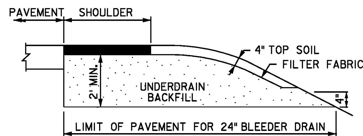
SECTION B-B
