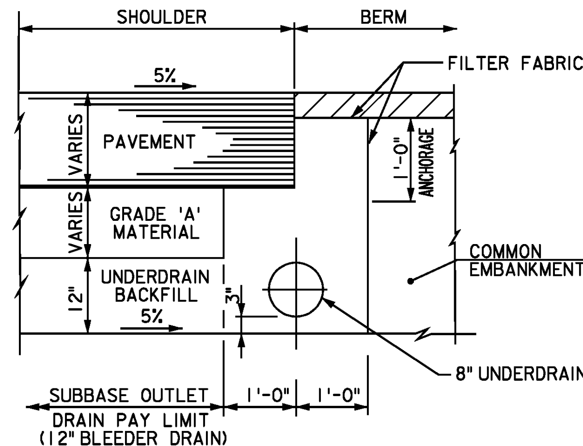
DETAIL 'B'
