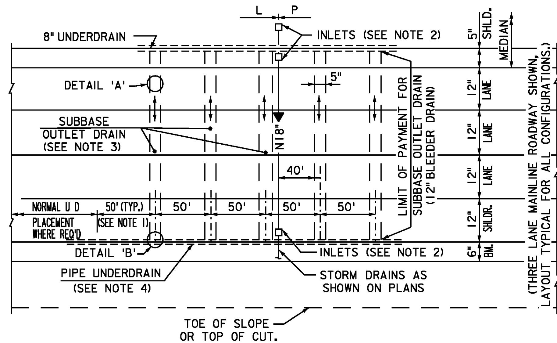
PLAN SUBBASE OUTLET DRAIN AT ROADWAY LOW POINT
