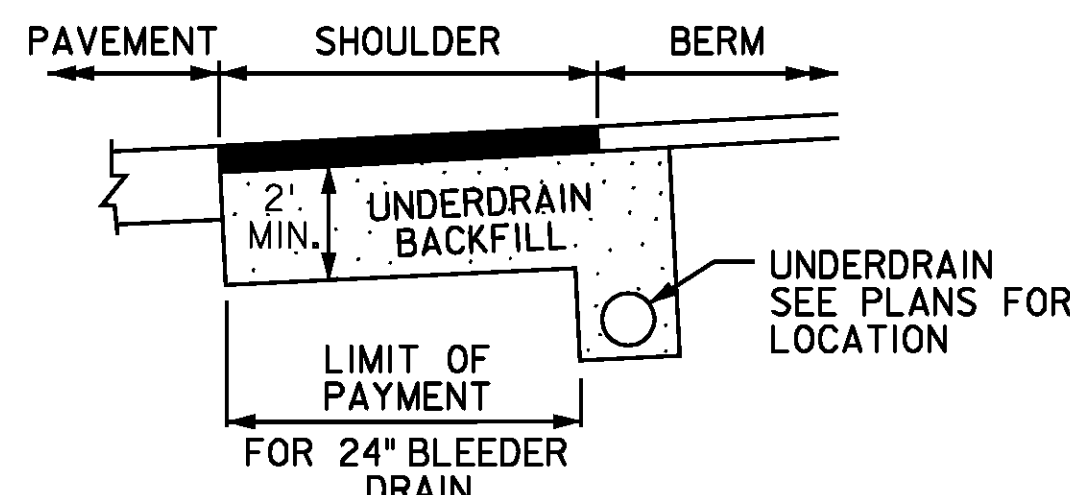
SECTION C-C
